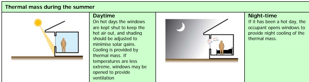
Figure 3b (continued on page 9) Passive cooling in summer, and storage and release of free energy gains in winter. (Courtesy of The Concrete Centre, UK )
